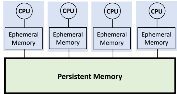
Figure 1: The Parallel Persistent Memory Model
